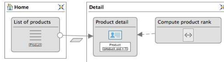
Figure 1. IFML model for an E-Commerce application
