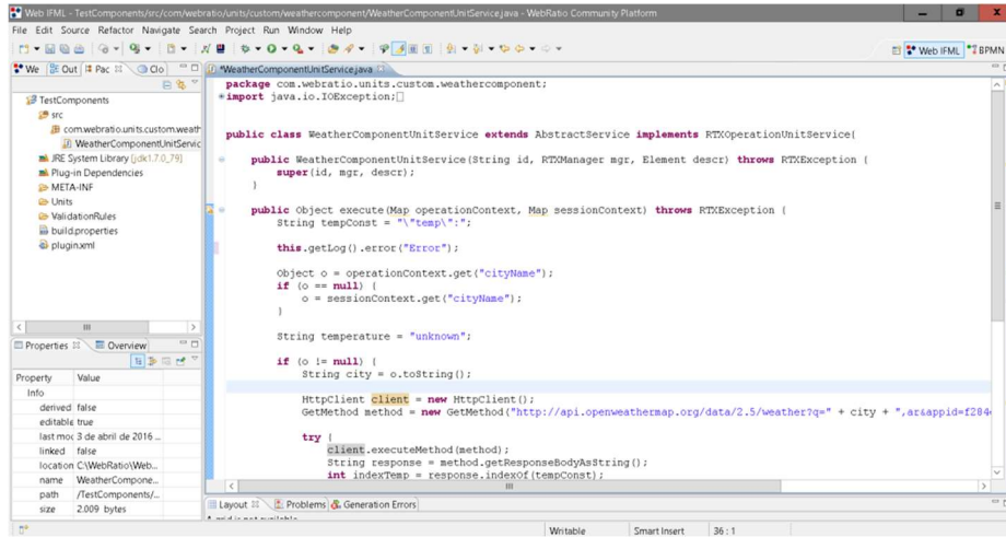
Figure 18. Implementation of the runtime java class for the custom Component.
