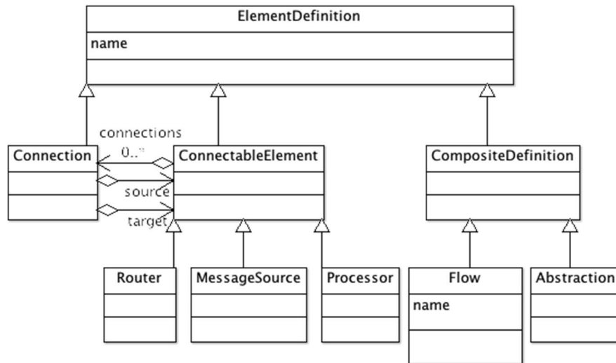
Figure 4. LiquidML metamodel
