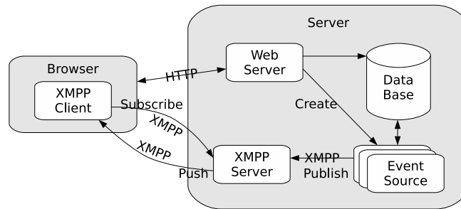
Fig. 3. The components of the Push System.
