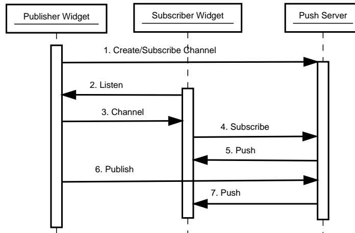
Fig. 2. The widget communication model.
