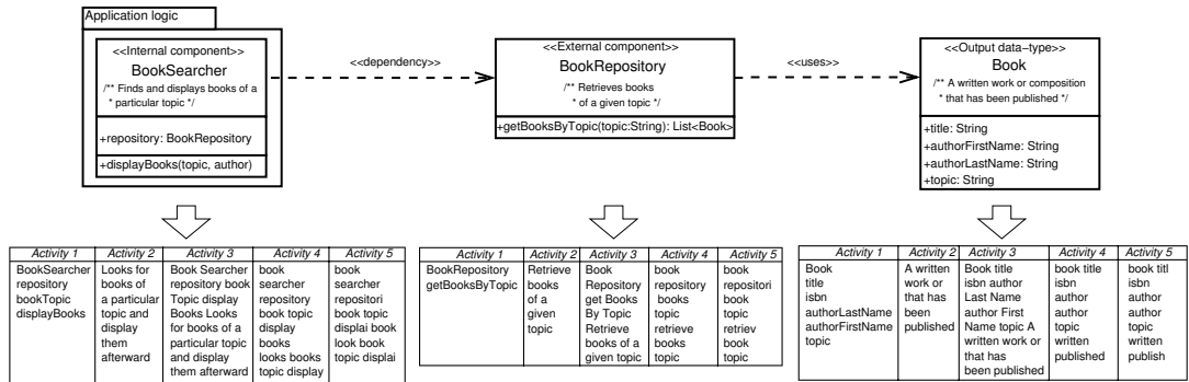
Fig. 4. Mining relevant terms from the book searcher example
