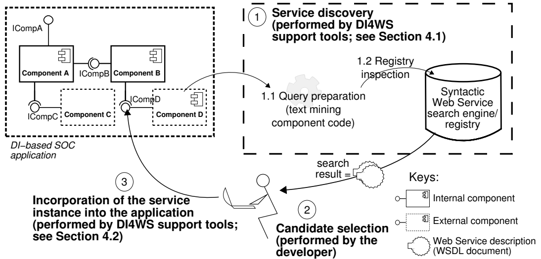
Fig. 3. Overview of DI4WS
