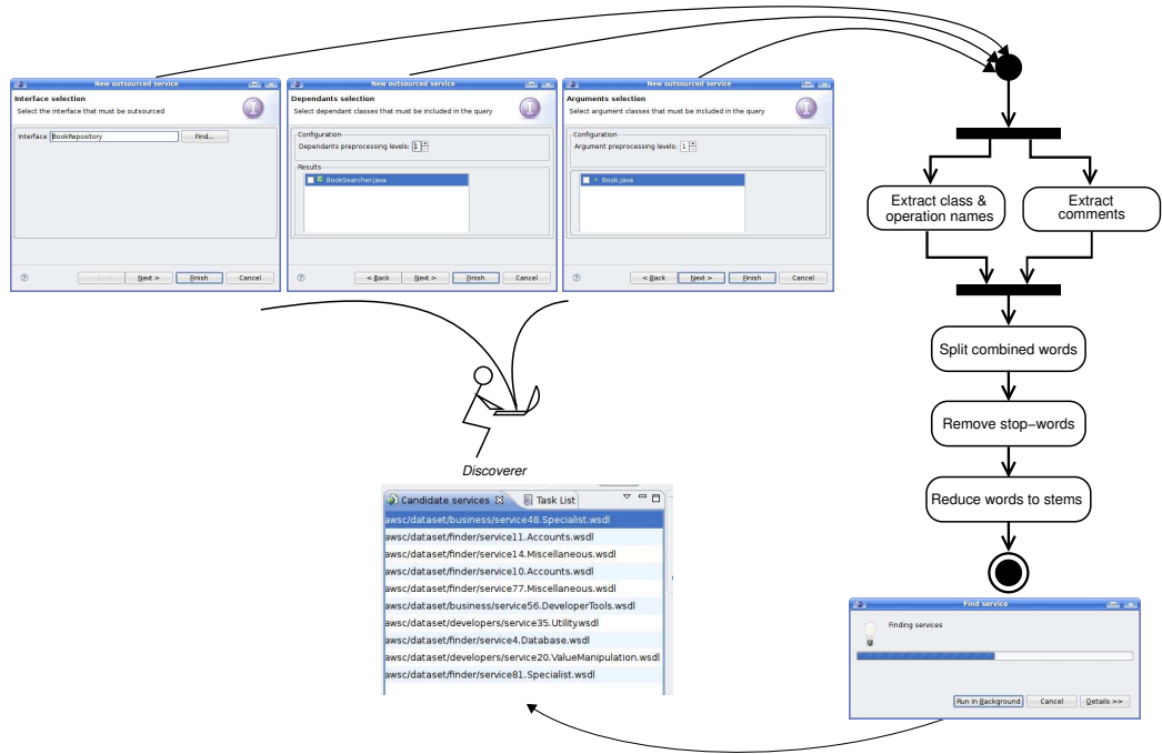
Fig. 5. The DI4WS Eclipse plug-in: Query generation and service selection
