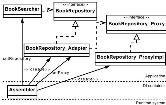
Fig. 7. The DI4WS book searcher application: class diagram
