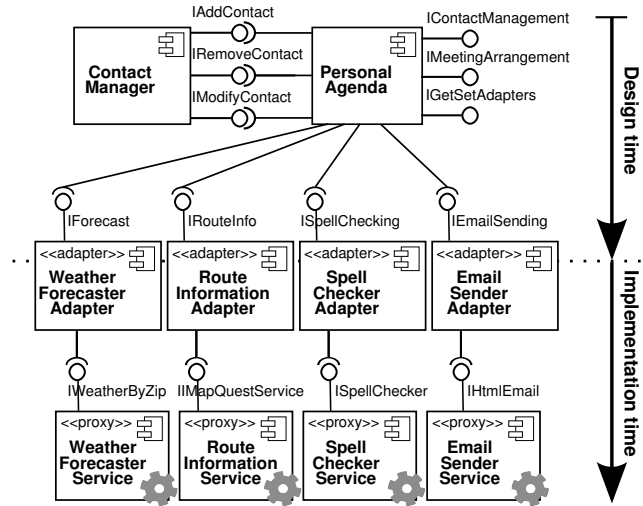
Fig. 11. Component diagram of the DI4WS implementation of the personal agenda
