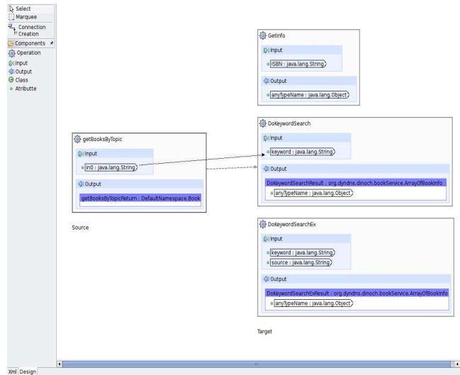
Fig. 8. The DI4WS Eclipse plug-in: Contract adaptation
