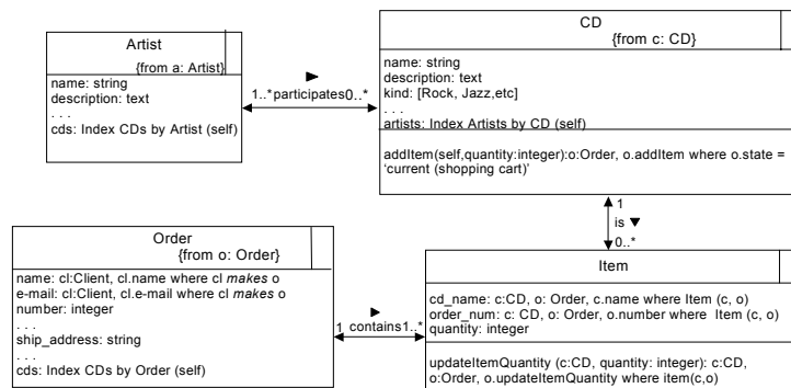
Figure 7 – The OOHDM navigational diagram (nodes and links) of the CD Store
