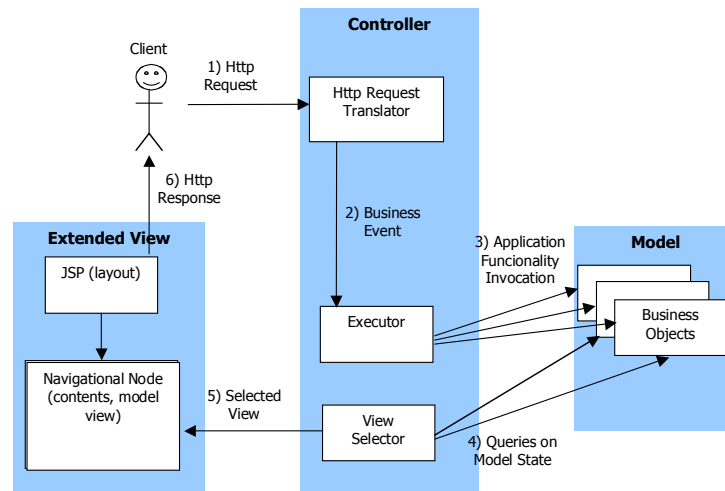
Figure 3: Main components of OOHDM-Java2
