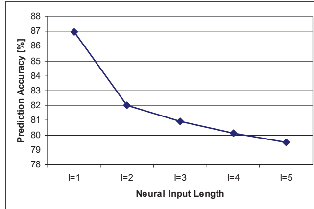
Figure 6 Varying the neural input length.
