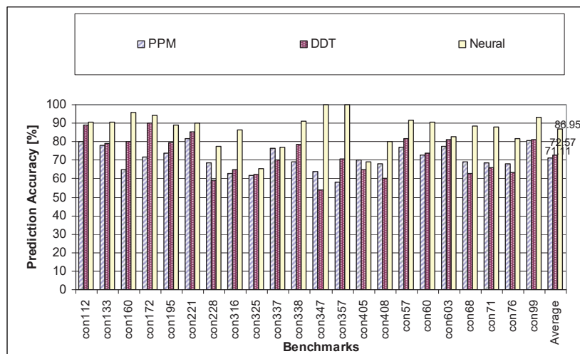
Figure 8 Comparing different hybrid web usage predictors.
