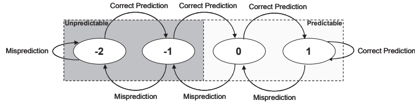
Figure 2 The 4-state confidence counter.
