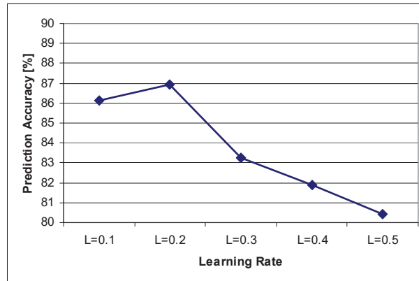
Figure 5 Varying the learning rate.
