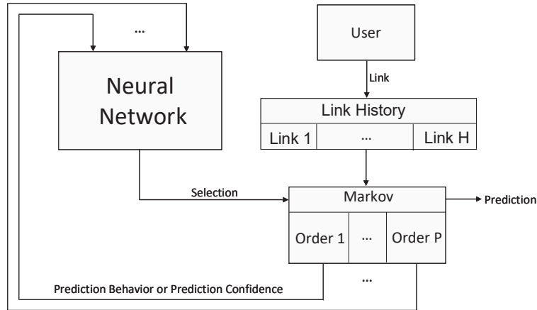
Figure 1 The structure of the browser extension.
