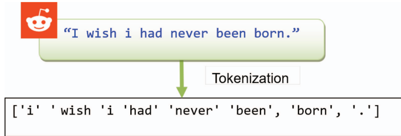
Figure 2 Tokenization example.
